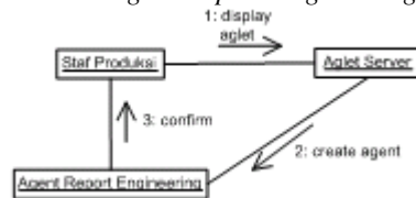
Gbr 6b Diagram Kolaborasi Create Agent Report Engineering
