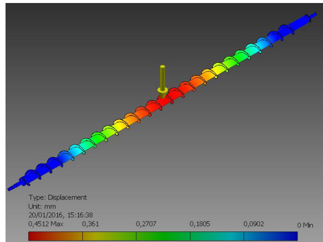
Gambar 4. Pengujian kelendutan assembly as flighting .
