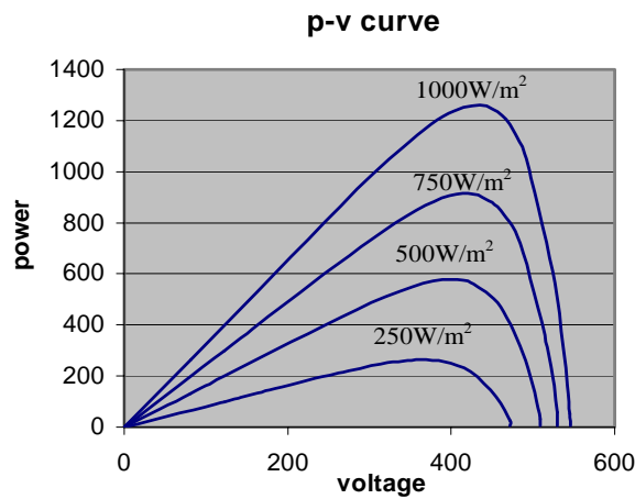
Figure 2. p - v curves of the PV array
