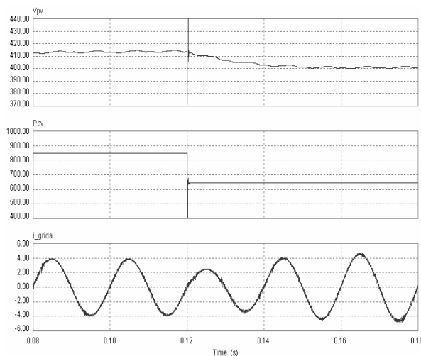
Figure 7. (Top to bottom) PV output voltage; PV output power; the grid current (phase A) when the insolation is changed ( 0.7\text{kW/m}^2 to 0.55\text{kW/m}^2 )
