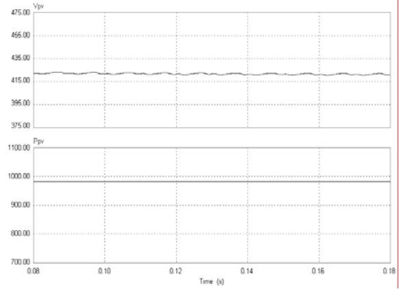
Figure 4. PV output voltage (top) and power (bottom) (for p_p = 0.8\text{kW/m}^2 )
