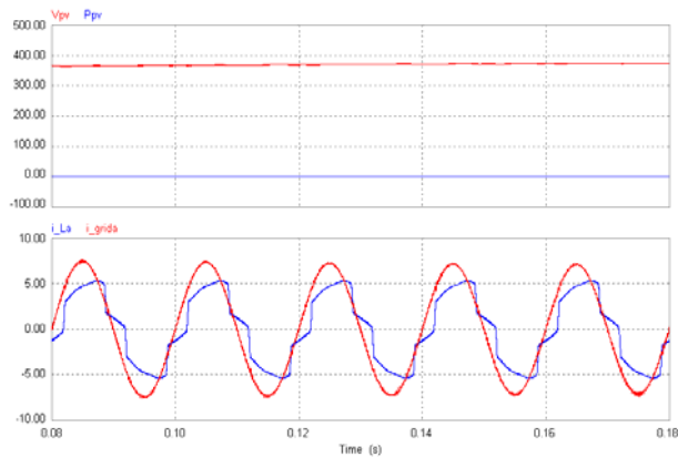
Figure 6. PV output voltage and power under zero insolation level (top); the grid and the load currents (bottom)
