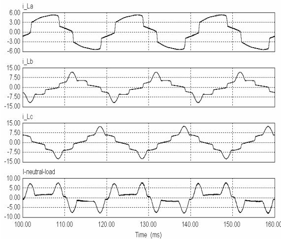
Figure 3. Mixed-load currents (phase a-b-c-neutral)
