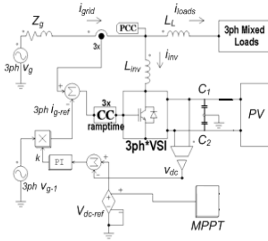
Figure 1. The proposed CC-VSI configuration
