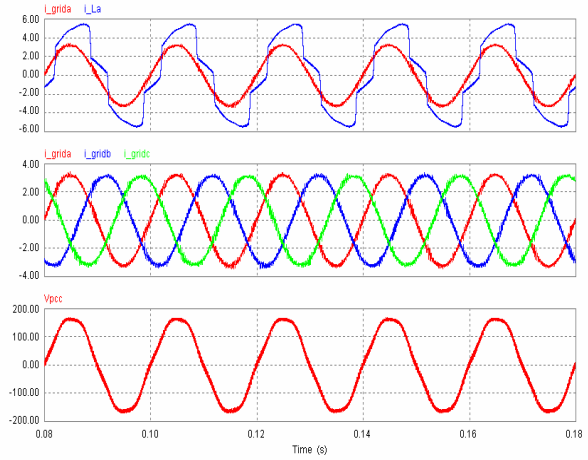
Figure 5. (Top to bottom) The grid and the load currents; three-phase grid currents; the grid voltage (phase A)
