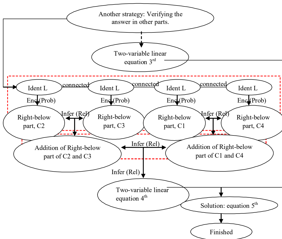
Figure 4. The Structure of S3' Analogical Reasoning after Verifying
