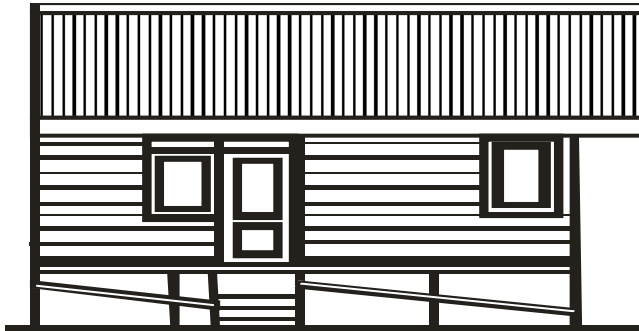
Fig. 7 Back Elevation Source: Purwanto (2008)
