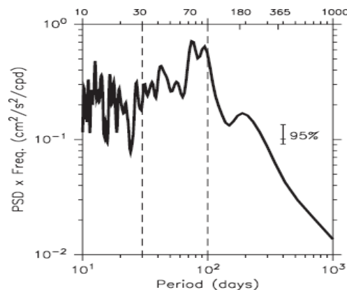
Fig. 3. Variance-preserving spectra of the observed zonal current shown in Fig. 2. at 1.5°S, 90°E for daily data.
