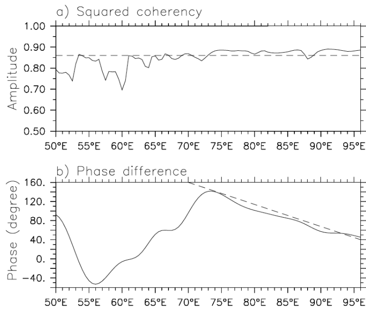
Fig. 5. Squared coherency amplitude (a) and phase (b) of the zonal current at 1.5°S, 90°E at 10m depth with the SSH at each longitude along the equator at period of 30 – 70 days. The dashed horizontal line in the upper panel is the 95% confidence level. The dashed line along the phase in the lower panel is a linear regression fit to time lag between 75°E and 95°E.
