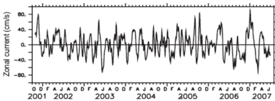
Fig. 2. Time-series of the daily zonal currents observed at 1.5°S, 90°E at 10 m depth.
