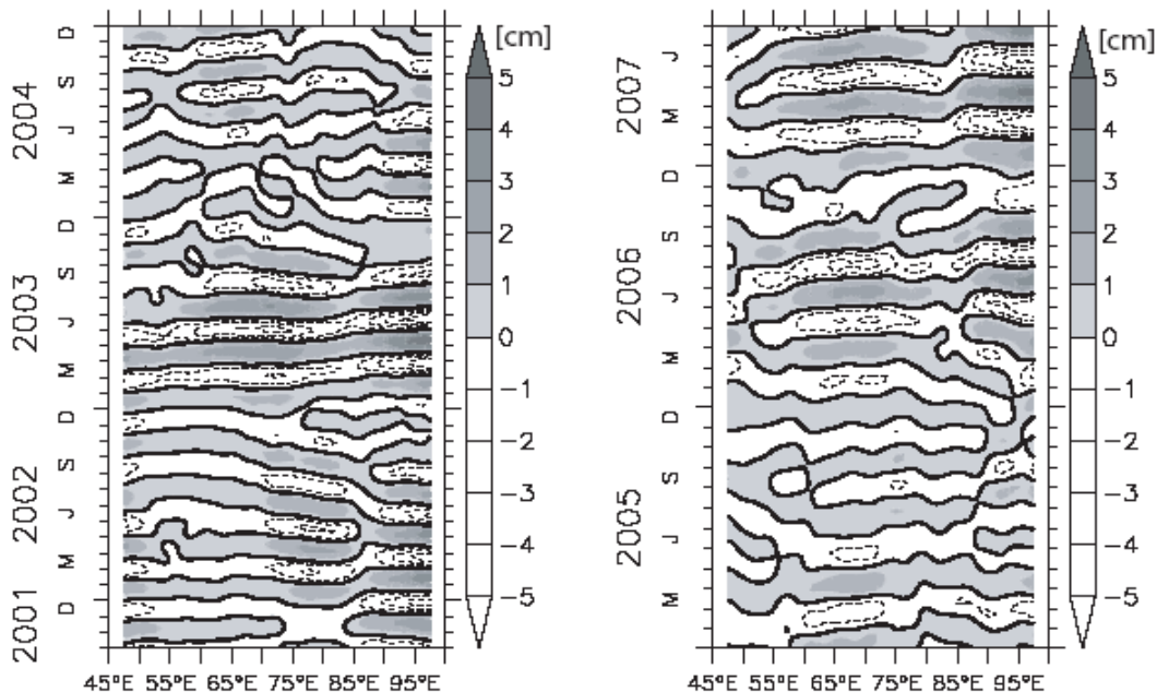
Fig. 6. Longitude-time diagram of the 30–70-days band-passed sea surface height along the equatorial Indian Ocean for the period of October 2001 through July 2007.
