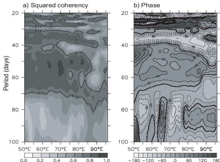
Fig. 4. Longitude-period plots of correlation between the equatorial zonal winds and the observed zonal current using the cross-spectral analysis. The left and the right panels indicate the squared coherency and the phase difference, respectively. The 95% confidence limit (0.73) is shown by thick contour in the left panel.
