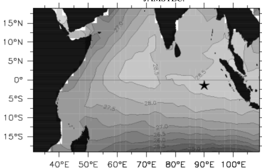
Fig. 1. Location of the TRITON buoy in the eastern Indian Ocean ( marked with STAR ) superimposed on the mean sea surface temperature from World Ocean Atlas 2001.
