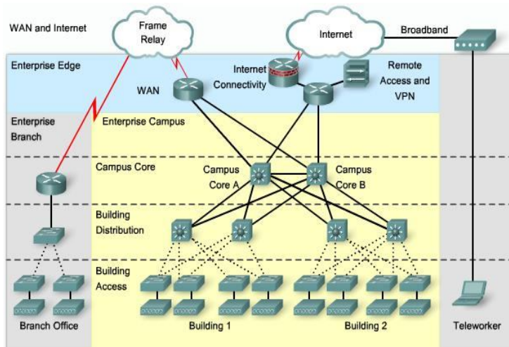
Gambar 4. Contoh Topology Enterprise Network (ideal)
