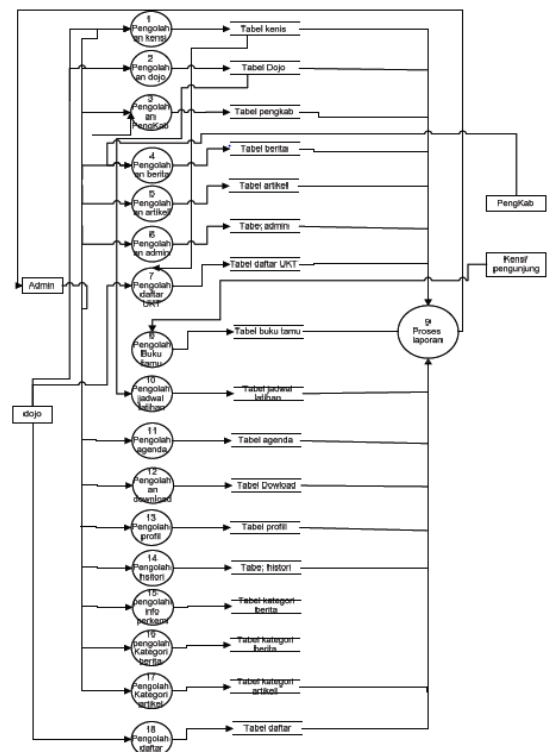
Gambar 4. DFD Level 1
