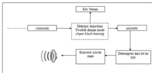
Gambar 4. Proses Dekripsi File Suara
