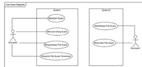
Gambar 5. Model Use Case
