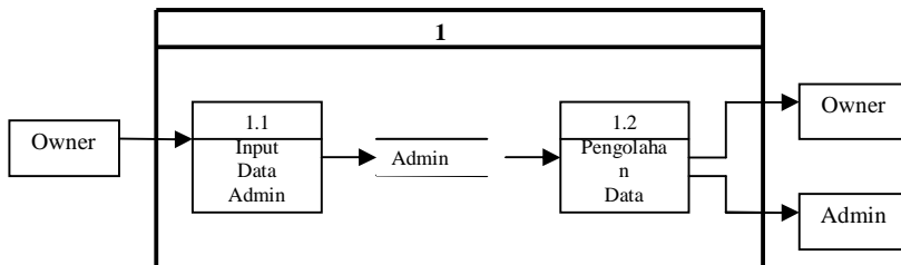
Gambar 3 Data Flow Diagram Level 2 Proses 2
