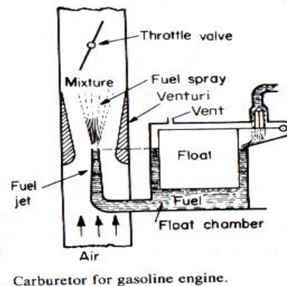
Gambar 2. Karburator
