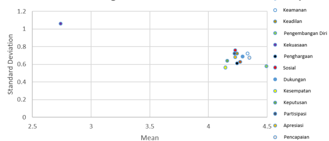
Gambar 3. Diagram Motivasi
