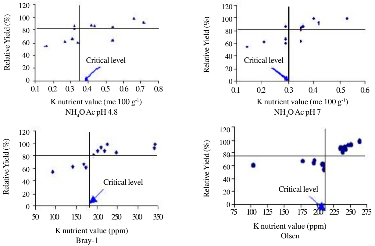
Figure 3. Critical level of K nutrient with graphs Cate Nelson and various K extractants.
