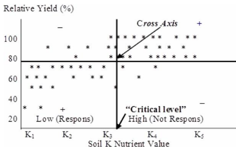
Figure 1. Graph Method of Cate-Nelson for Ascertainment of Availability K Nutrient Class
