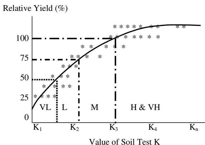
Figure 2. Continuous Curve Method for Ascertainment of Availability K Nutrient Class. VL: Very Low, L: Low, M: Moderate, H: High, VH: Very High.
