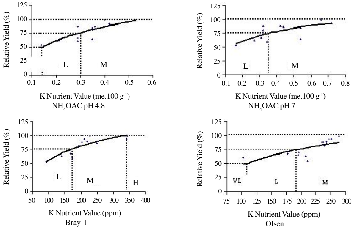
Figure 4. Availability class of K nutrient by continuous curve method on various extractants.
