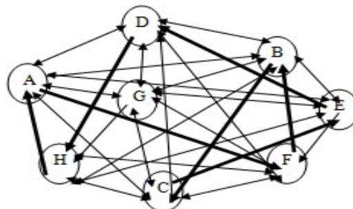
Gambar 5. Graf Lintasan Distribusi Hari Senin Metode Nearest Neighbour
