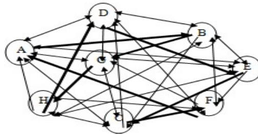
Gambar 4. Graf Lintasan Distribusi Hari Senin Metode Branch and Bound
