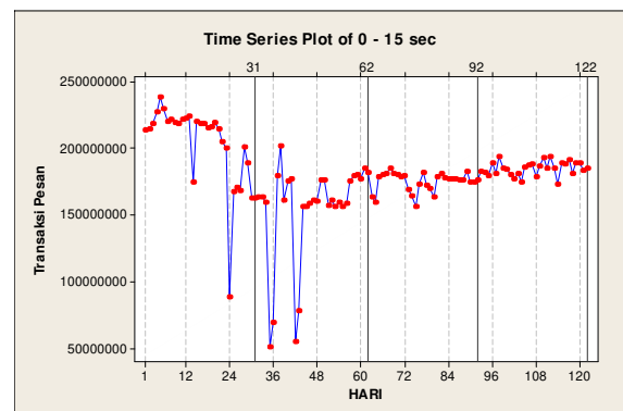
Gambar 3. Grafik Time Series Plot All Operator 0-15 sec
