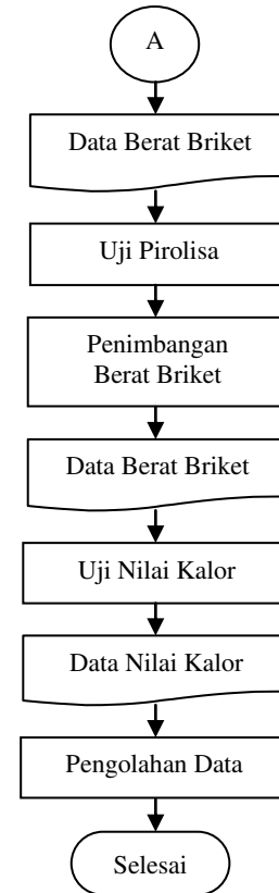
Gambar 1. Flowchart Penelitian Uji Nilai Kalor Briket Biomassa.
