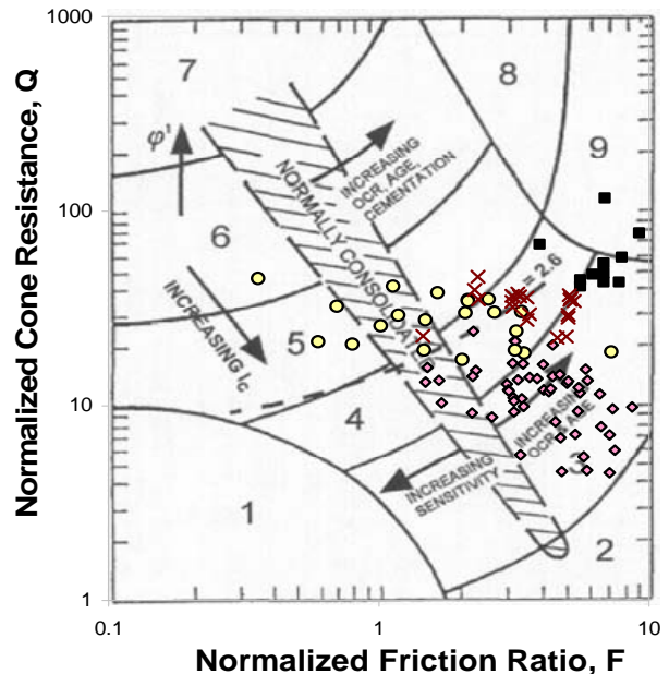
Figure 2. Q-F analysis for Location A
