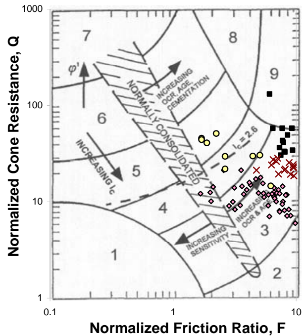
Figure 4. Q-F analysis for Location B (■: 0-3 m, ×: 3.0-7.5m, ◇: 7.5-20.0m, ○: >20m)
