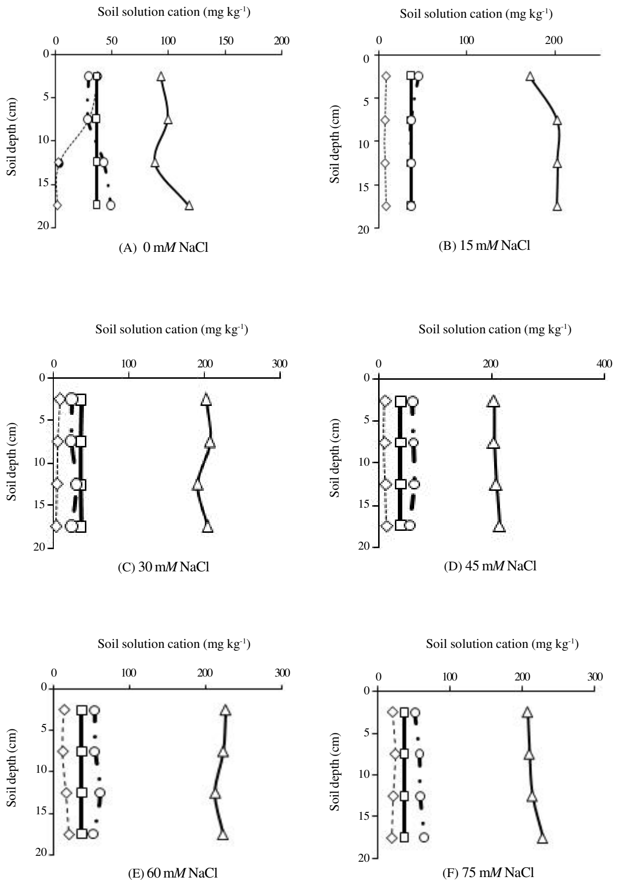
Figure 1. Cations dynamics in 0-20 cm soil depht after harvest on varion dosages of NaCl. ---◇--- = K, —□— = Na, —△— = Ca, and ---○--- = Mg.
