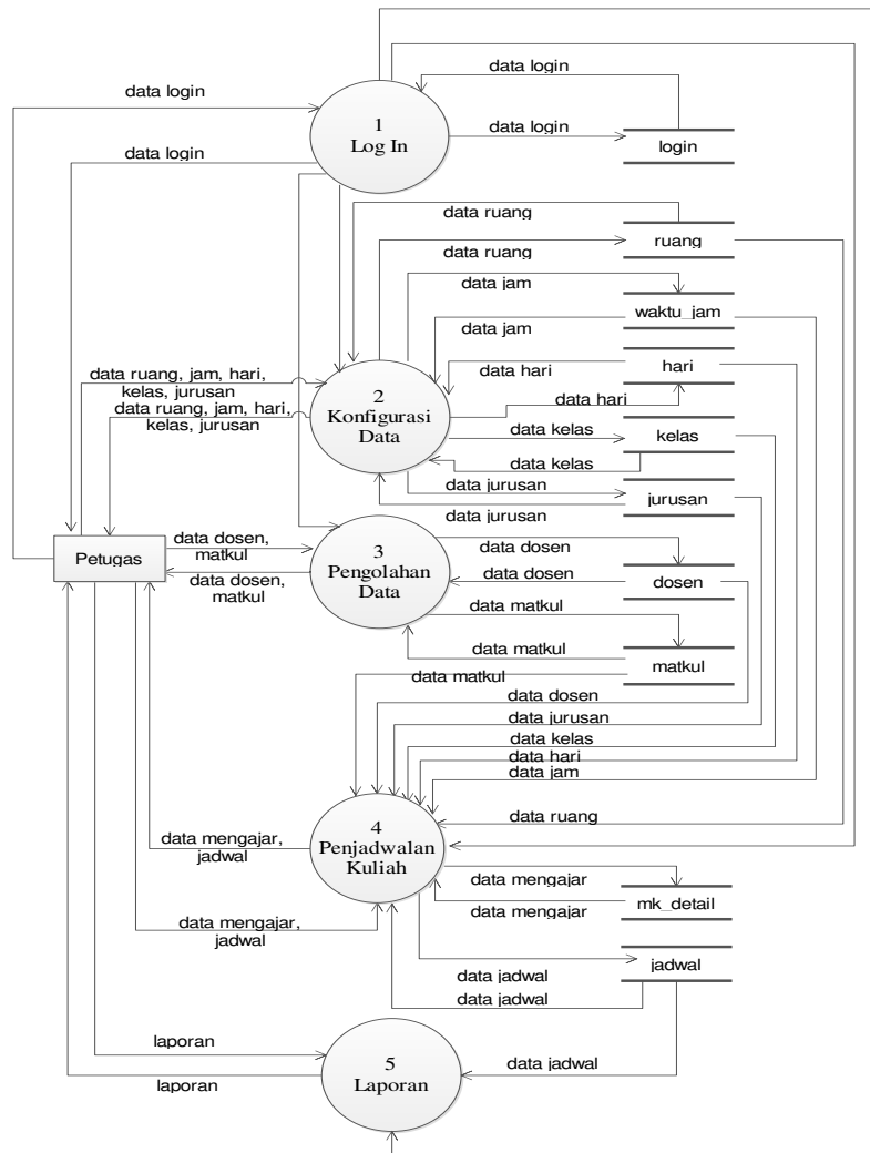
Gambar 4. Diagram Level 1
