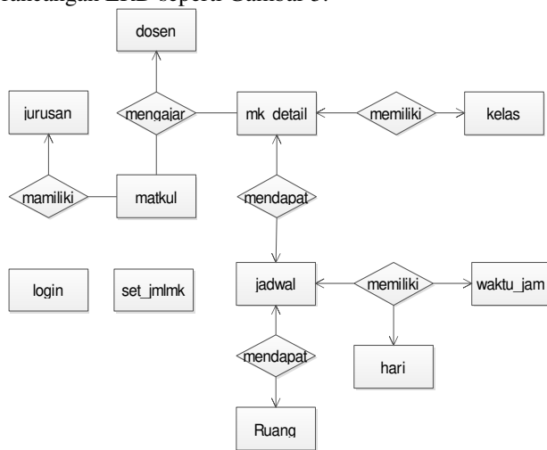
Gambar 5. Entity Relationship Diagram
