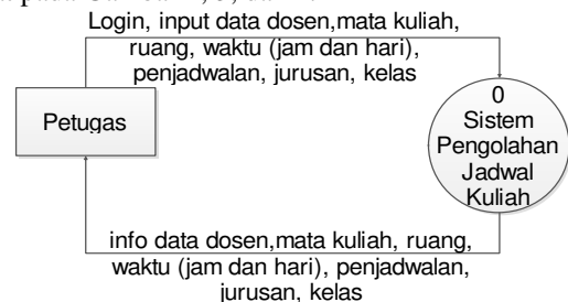
Gambar 2. Diagram Konteks (Diagram level 0)
