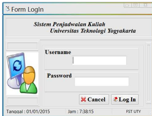
Gambar 7. Form Login
