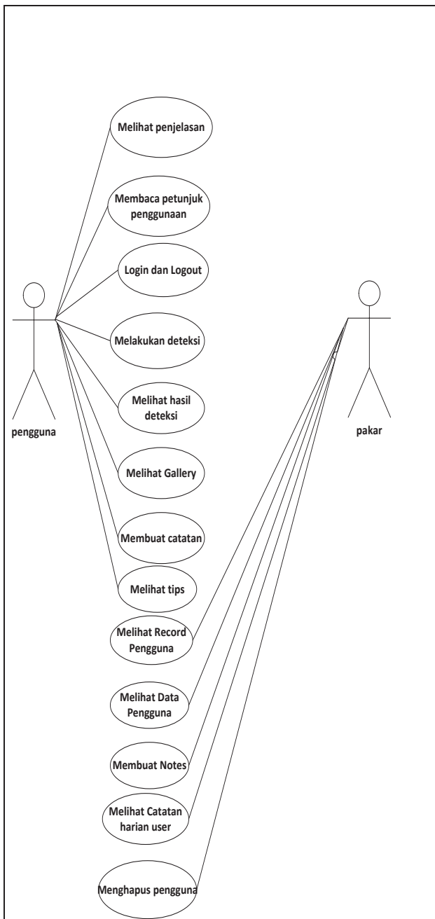
Gambar 3 Use Case Diagram
