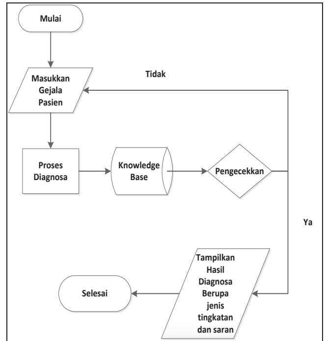
Gambar 2 Flowchart Mekanisme Inferensi Forward Chaining
