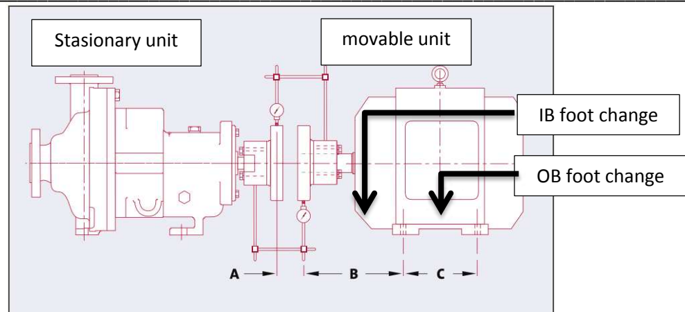
Gambar 3. Metode reverse dial indicator
