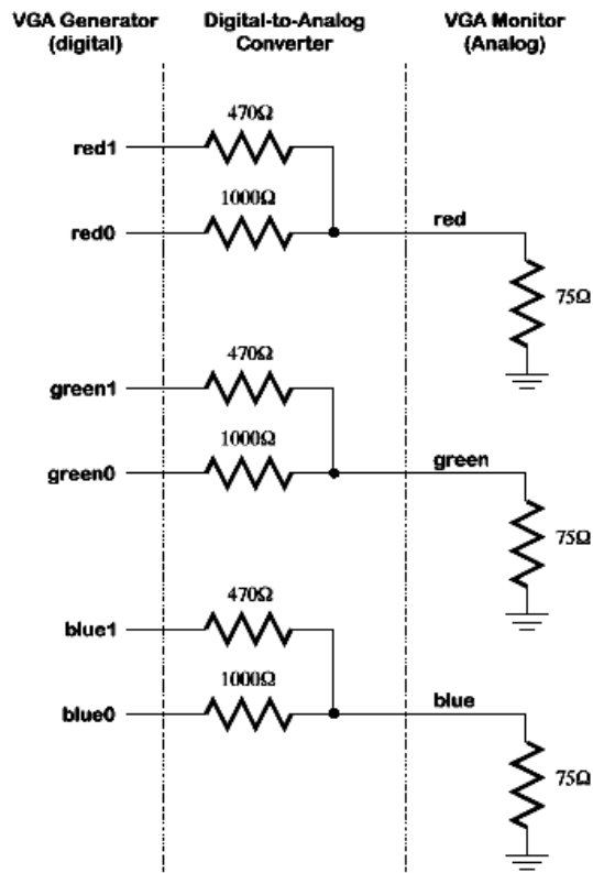
Figure 2. Digital to analog VGA monitor interface [2]
