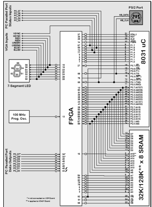
Figure 4. Interconnect diagram within XS-40. [4]
