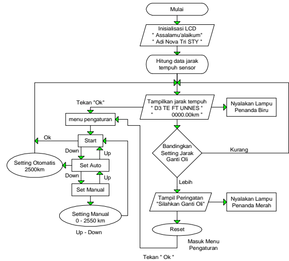
Gambar 10. Diagram Alir Kerja Program
