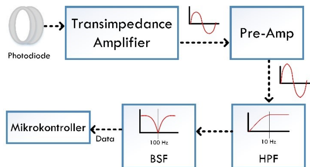
Gambar 4. Rangkaian AFE Receiver
