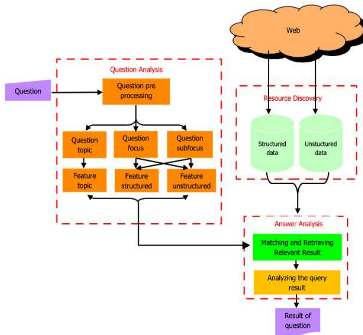
Figure 3. Framework of finding structured and unstructured features to improve result of complex questions.
