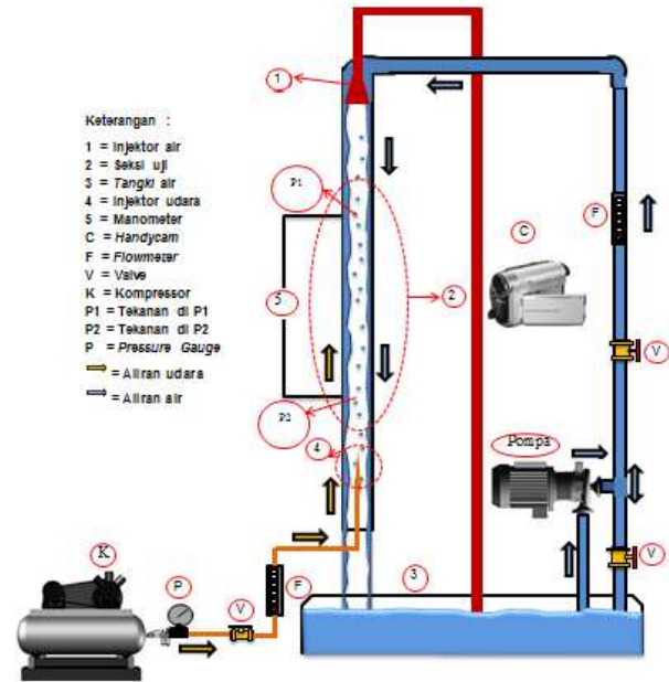
Gambar 1. Instalasi penelitian.
