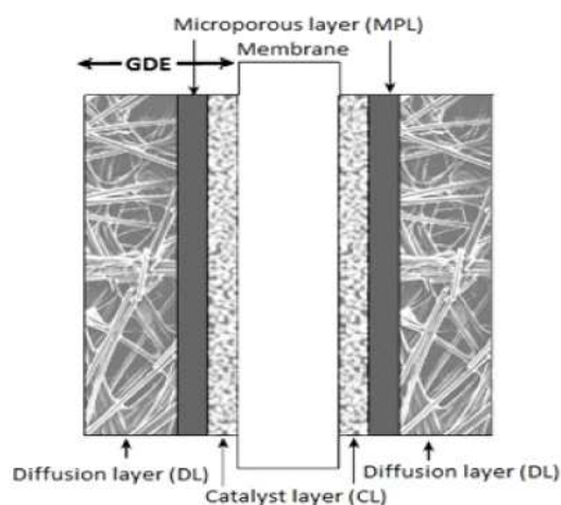
Figure 1. Schematic of MEA and its components [5]
