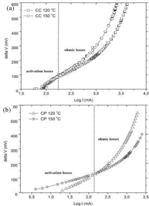
Figure 5. Tafel plot of both GDE based on (a). carbon cloth and (b). carbon paper
