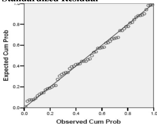
Gambar 5.1 Normal Probability Plot
