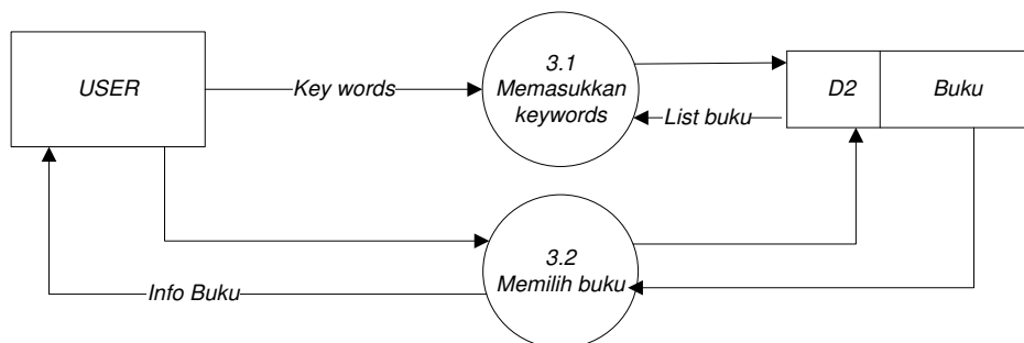
Gambar 4 DFD Level 1 Proses Search
