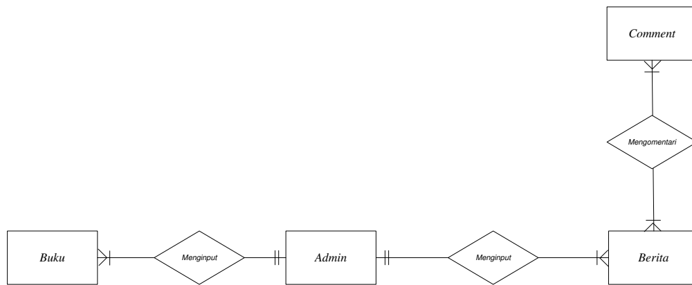
Gambar 6 Entity Relationship Diagram
