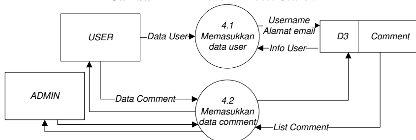
Gambar 5 DFD Level 1 Proses Leave Comment
