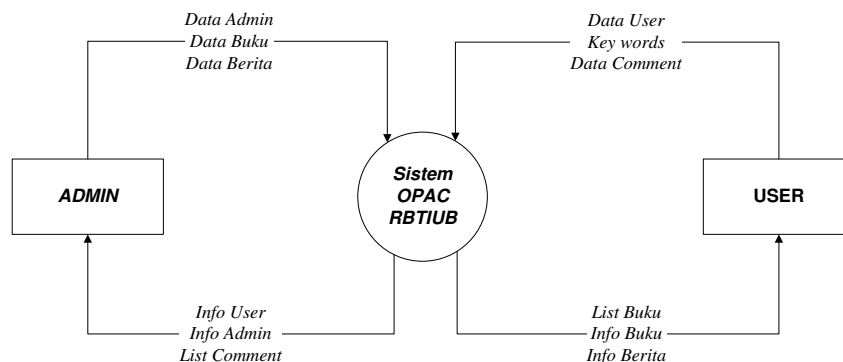
Gambar 1 Context Diagram
