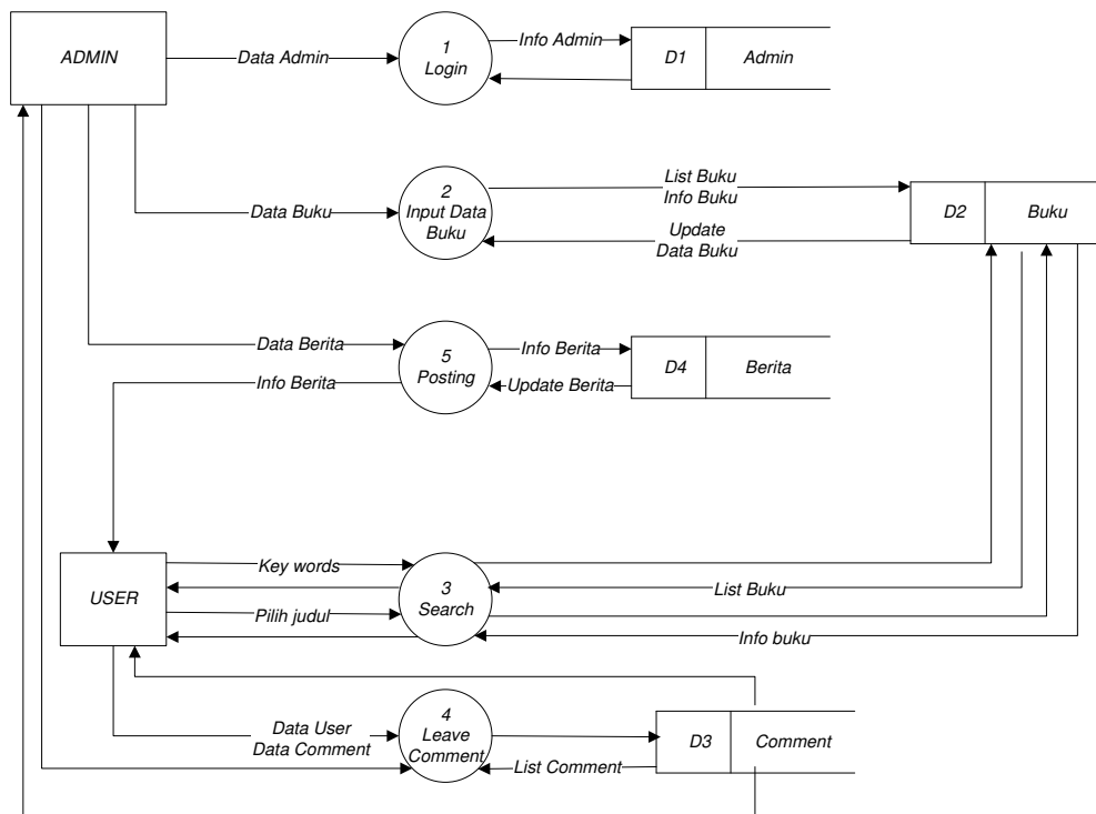
Gambar 3 DFD Level 0
