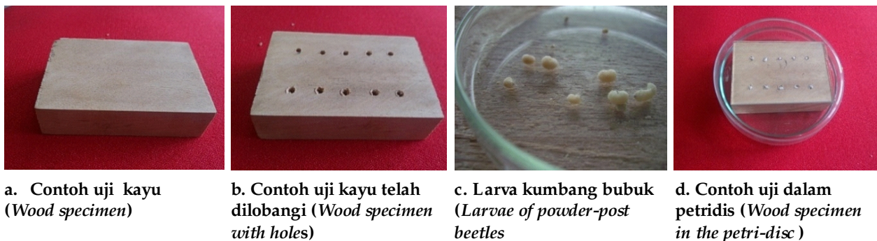
Gambar 1. Proses pengujian kayu terhadap kumbang bubuk Figure 1. The testing process of wood against powder-post beetle
