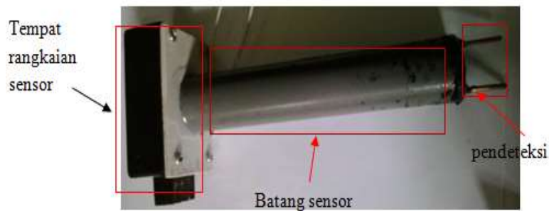
Gambar 5. Sensor salinitas
