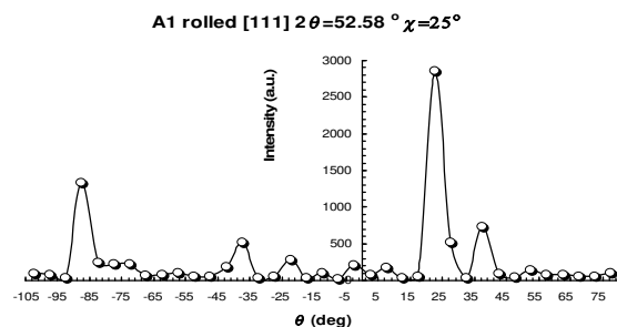
Figure 4. 0-2\theta scan of a hot rolled A1 LCS taken in the [111] ( 2\theta=52.58^\circ ) crystallographic direction and \chi=25^\circ
