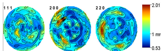
Figure 7. Pole figure for the hot-rolled A1 LCS specimen ODF resolution of 5^\circ
