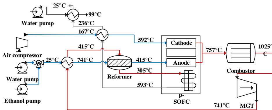
Figure 2. Case 2 with fuel heater before reformer.
