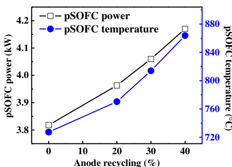
Figure 7. Anode recycling effect on pSOFC power and temperature.
