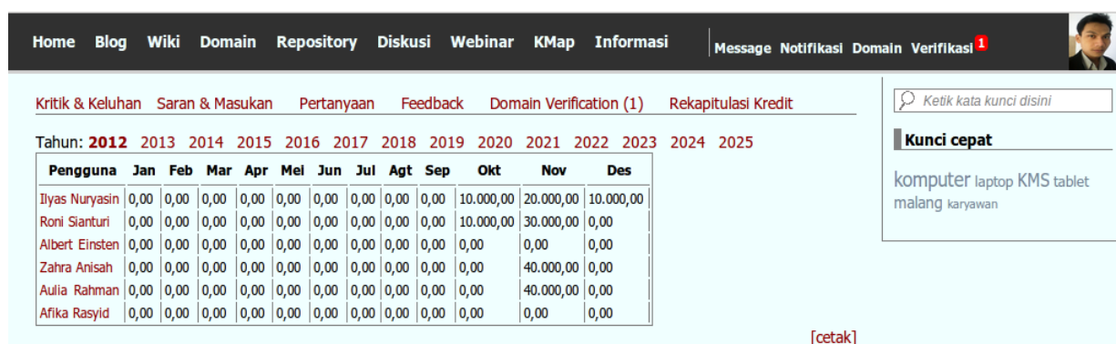
Figure 7. User Credit
