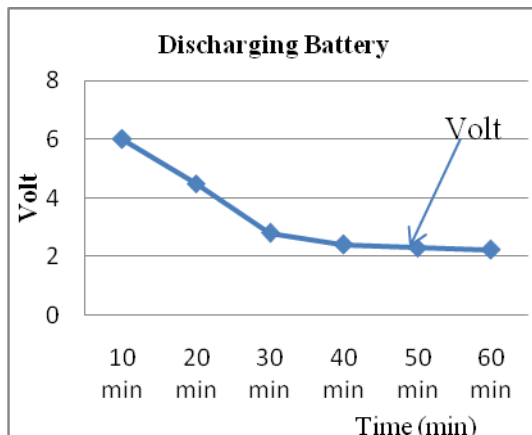
Figure 7. Discharger Volt Battery.
