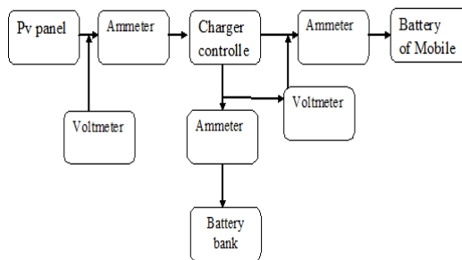
Figure 10. Measurement diagram.
