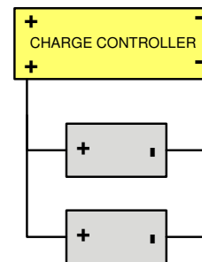
Figure 5. Battery Bank in parallel.
