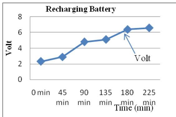
Figure 6. Overcharge volt battery.
