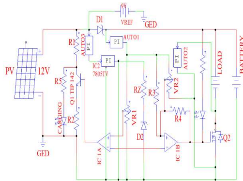
Figure 9. Charge Controller Circuit.
