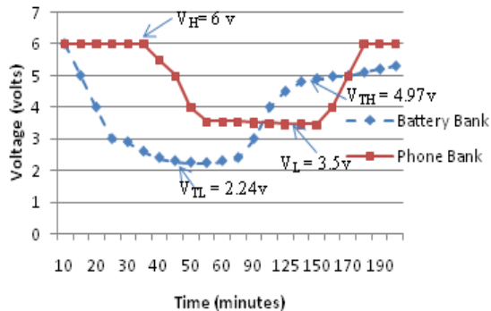
Figure 12. Discharge control using Schmitt Trigger.
