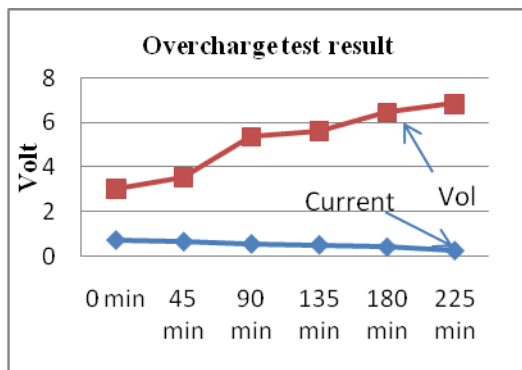
Figure 11. Overcharge test result.
