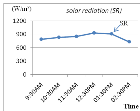
Figure 3. Variation in intensity of solar radiation with time.
