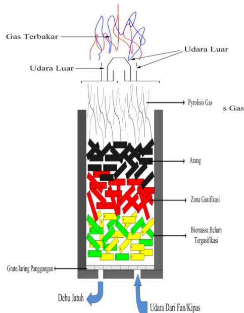
Gambar 1. Model Proses
