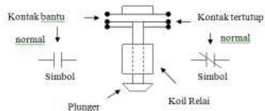
Gambar 1. Relai elektromekanis
