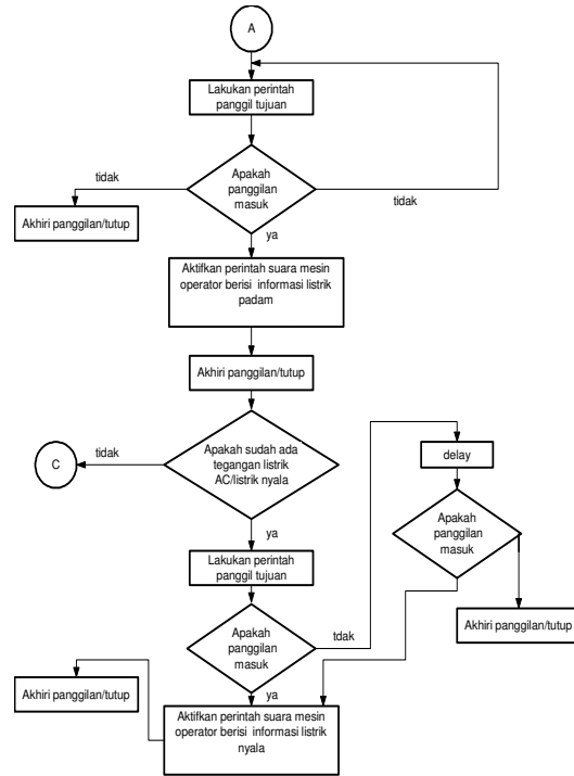
Gambar 14. Flowchart Program Sub Rutin A
