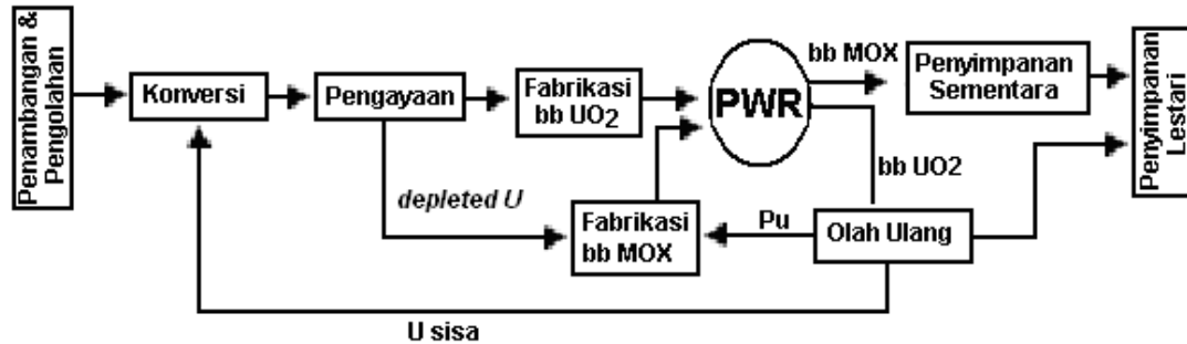
Gambar 2. Opsi Daer PWR-MOX [3,4,5]
