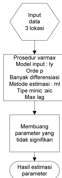
Gambar 2. Flowchart prosedur VARIMA
