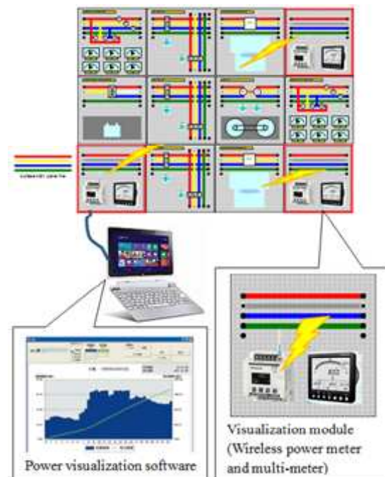
Figure 3. Visualization of Electric Power by Module-Type Power System Training Device
