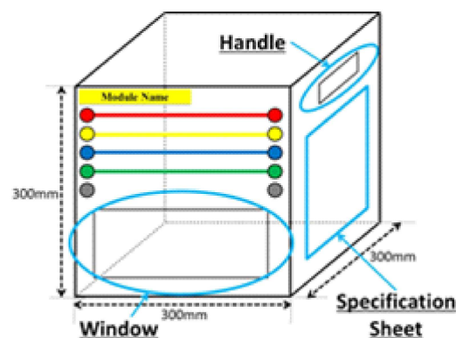
Figure 1. Standard of Module-Type Power System Training Device
