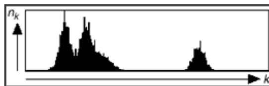
Gambar 1. Histogram citra
