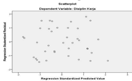
Gambar 4 Scatterplot
