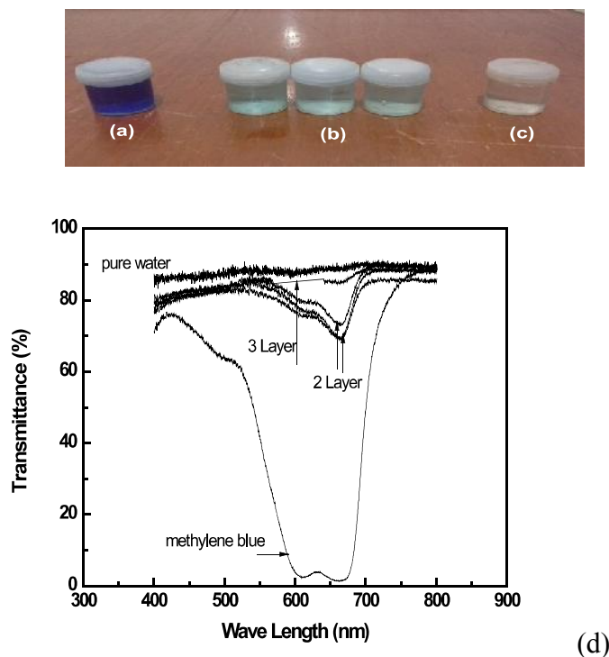
Figure 6. (a). Methylene blue solution; the results of water filtration process in porous composite (b) double layered, (c) triple layered; and (d) absorption spectrum from the water results of filtration process.
