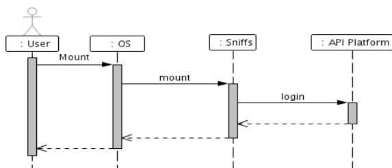
Gambar 6. Sequence Diagram Proses Mounting
