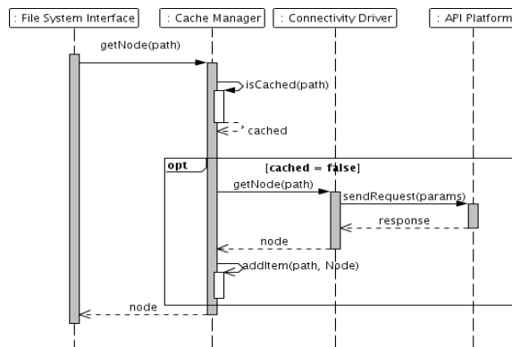
Gambar 3. Sequence Diagram Pengambilan Node
