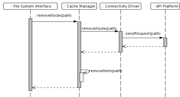
Gambar 5. Sequence Diagram Penghapusan Node
