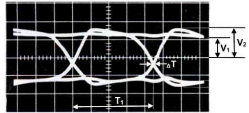
Gambar 3. Eye Pattern [12]
