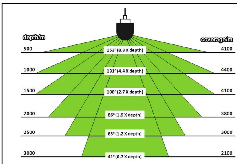
Gambar 2. Lebar sapuan Multibeam Echosounder Elac Seabeam 1050D (L3 Communications Elac Nautik).
