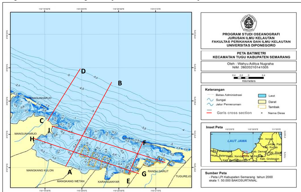
Gambar 3. Peta Batimetri garis cross section
