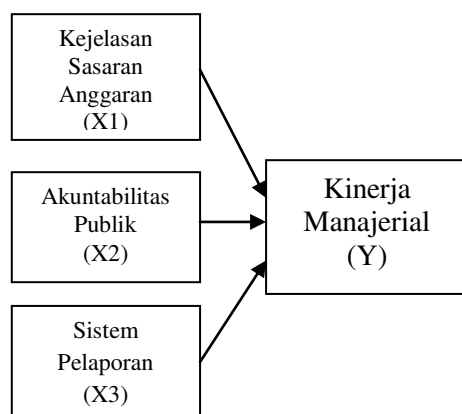
Gambar1 Model Penelitian
