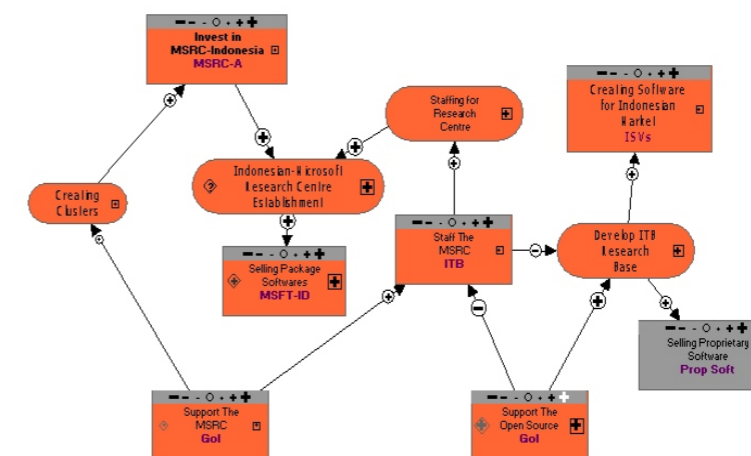
Exhibit 9 Model for DANA Analysis
