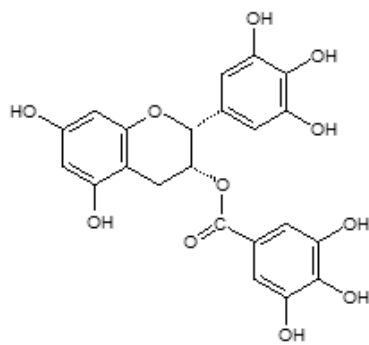
Figure 1. Structure of (-)-epigallocatechin gallate (EGCG) from green tea.
